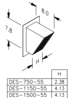
REACTIVATION OUTLET HOOD w/SCREEN
