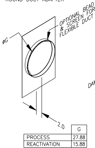
PROCESS & REACTIVATION INLET ROUND DUCT ADAPTER
