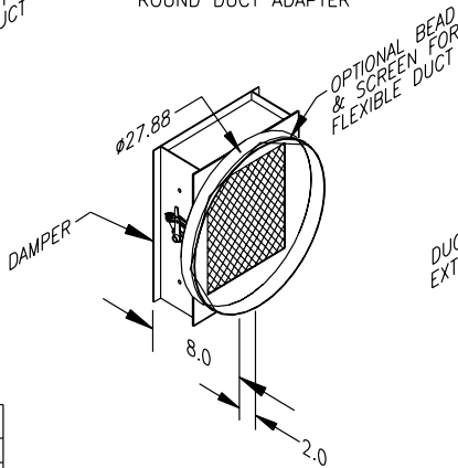
PROCESS OUTLET ROUND DUCT ADAPTER
