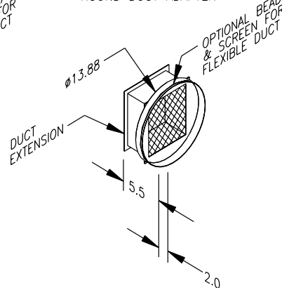
REACTIVATION OUTLET ROUND DUCT ADAPTER
