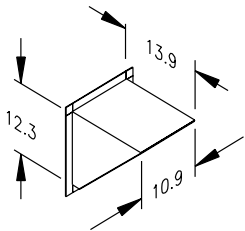
REACTIVATION OUTLET HOOD WITH SCREEN
